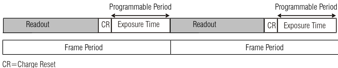
Figure 15: Mode 8 Timing
