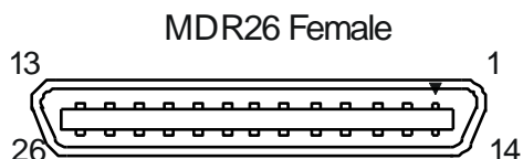
Figure 6: Camera Link MDR26 Connector
