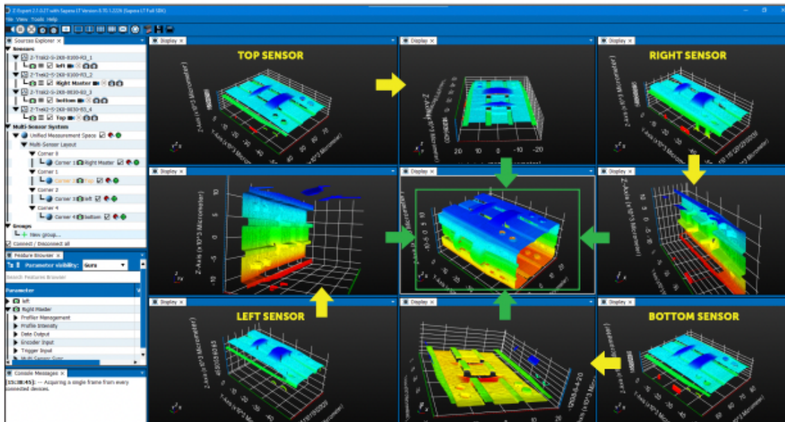
Z-Expert 360° View Using 4 Synchronized Z-Trak Sensors
